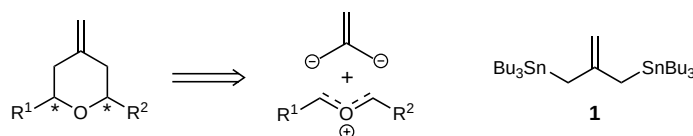
Scheme 1. General protocol for the synthesis of a tetrahydropyran by means of sequential allylic transfer reactions.
